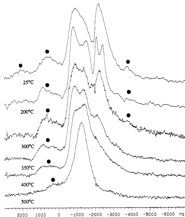
Figure 6. 29 Na MAS NMR spectra of synthetic nepheline (Na 0.75 (Na 0.20 K 0.05 )AlSiO 4 ) at high temperature. Spinning side bands are marked by solid circles.
