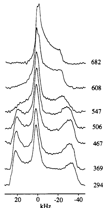
Figure 5. ^{23}\text{Na} NMR spectra of dehydrated zeolite \text{K}_6\text{Na}_6\text{-A} . Temperatures in kelvin are shown (reprinted from ref 18; copyright 1989 American Chemical Society).
