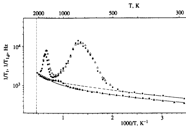
Figure 15. 1/T_1 (solid triangles) and 1/T_{1\rho} (other symbols) for ^{51}\text{V} in polycrystalline vanadium metal, plotted against inverse temperature. Dashed line shows melting point (reprinted from ref 24; copyright 1983 Pergamon Press).
