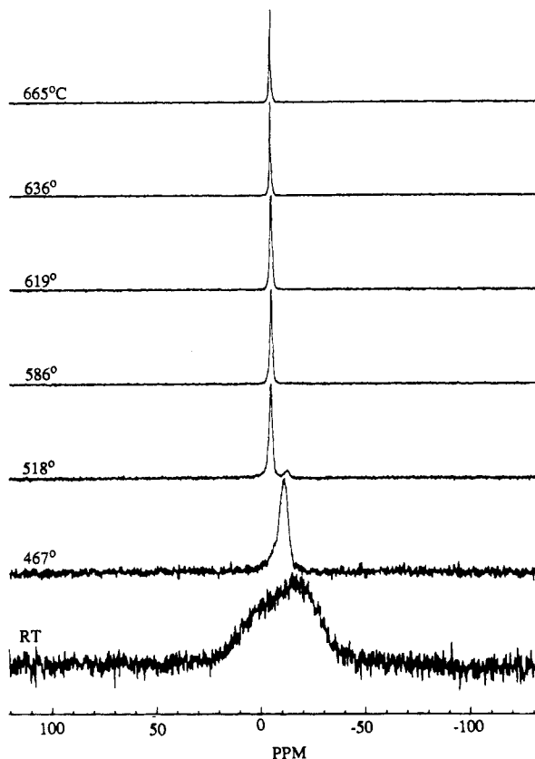
Figure 10. High-temperature ^{23}\text{Na} spectra for \text{LiNaSO}_4 . At 518 ^\circ\text{C} , most of the sample has transformed to the superionic conductor phase. Above 620 ^\circ\text{C} , the material is completely molten and shows a further decrease in line width (reprinted from ref 172; copyright 1990 Elsevier Scientific Publishers).
